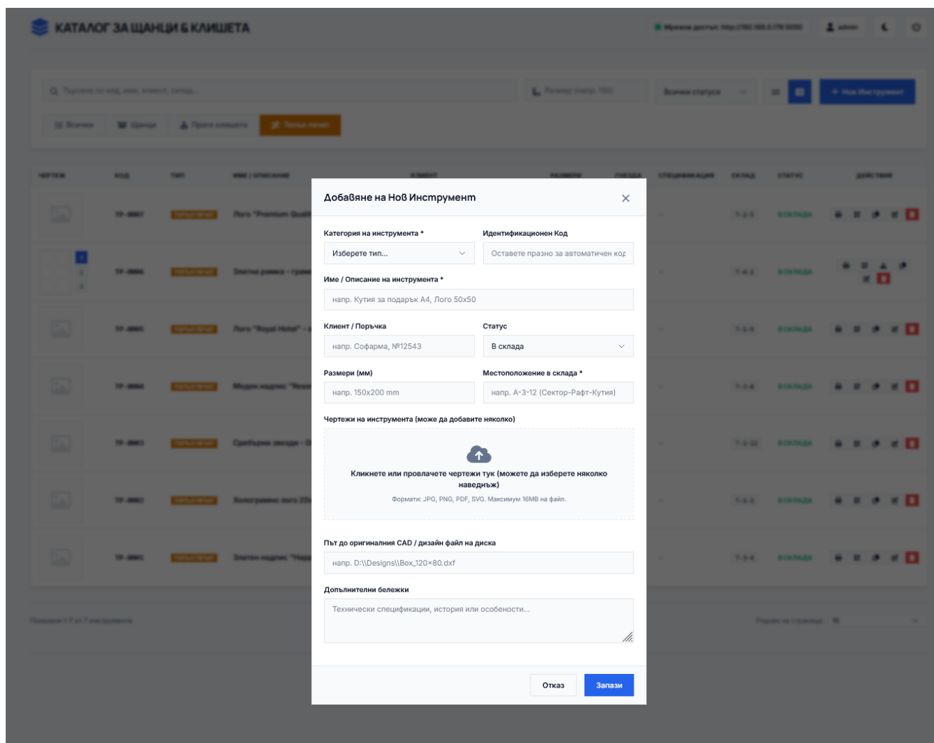
Application screen 2
